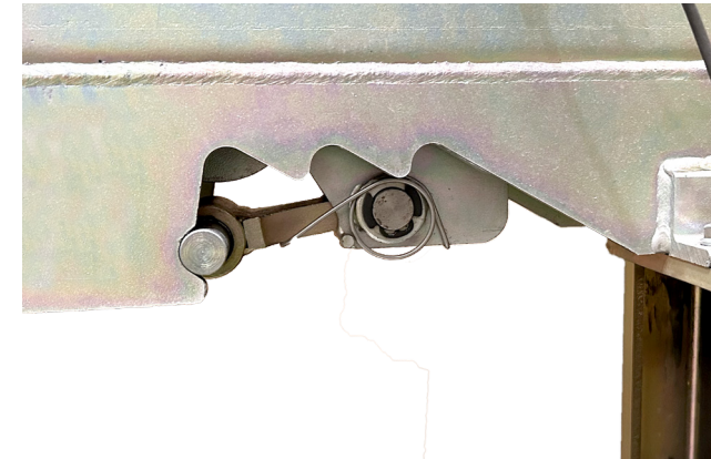
3-position slide lock limits trailer movement
